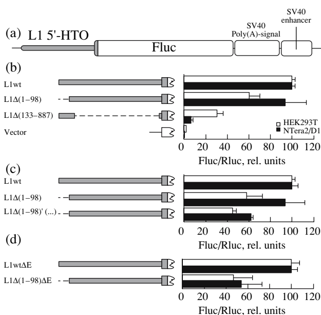
Fig. 2. Contribution of the minimal promoter into the total L1 transcription efficiency. (a) Structure of the L1wt construct. (b) Structures of the 5'-UTR constructs L1wt, L1 \Delta (1–98), and L1 \Delta (133–887) and pRF \Delta SV40 used as a negative control (on the left) and relative luciferase activity during the expression of the constructs in the cell culture (on the right). The pRluc plasmid, expressing the Renilla luciferase gene ( Rluc ) under the SV40 promoter, was taken as a normalizing vector. For each construct, the Fluc/Rluc values were normalized by the L1wt values. Each experiment was repeated at least three times. (c) The result of deletion of the 100 5'-terminal nucleotides does not depend on the adjacent sequence; the designations are as in Fig. 2b. (d) The result of deletion of the 100 5'-terminal nucleotides does not depend on the presence of the SV40 enhancer in the plasmid; Fluc/Rluc values were normalized by the values obtained for L1wt \Delta E.
